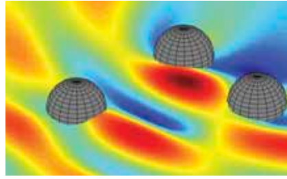
Modelling free surface elevations around floating structures
