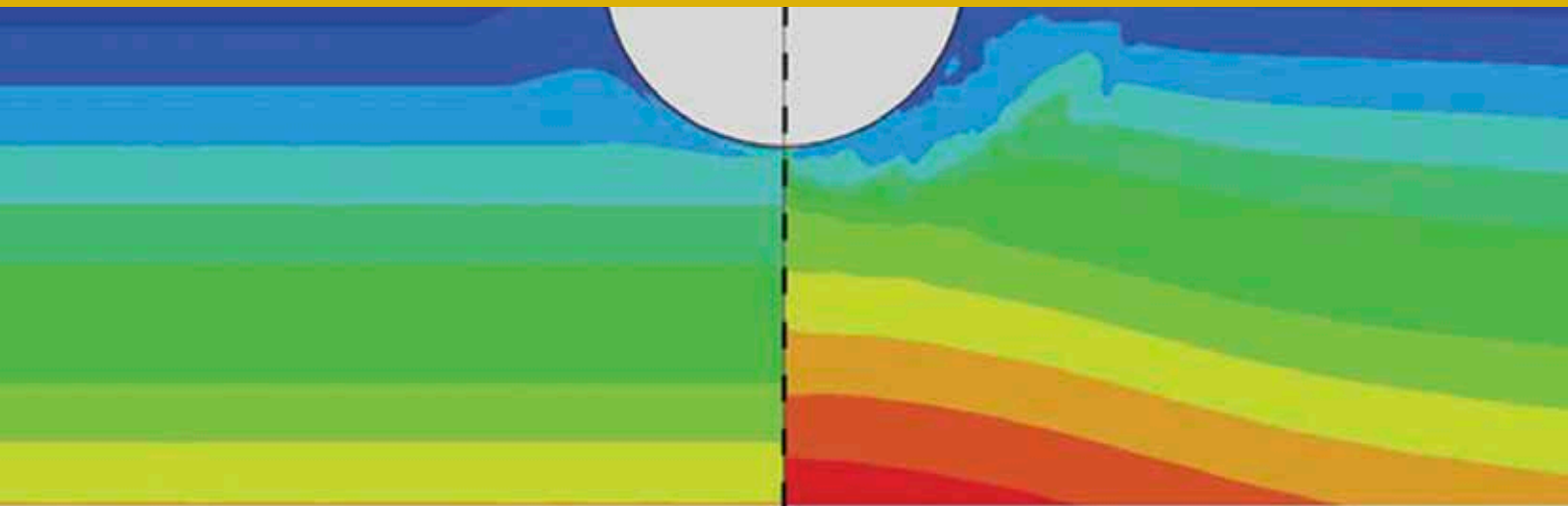
Modelling seabed softening and rate effects during pipeline penetration
